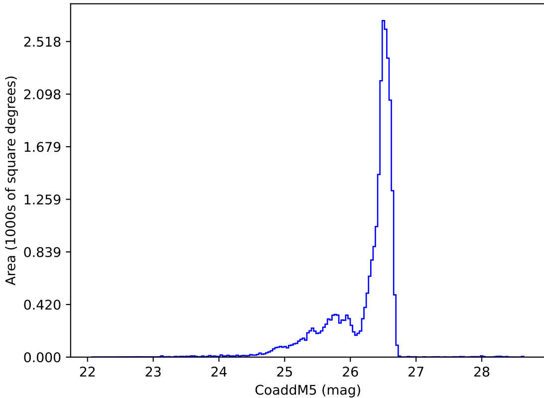
ddf_acor_sf10_lsf30_lsr20_v3.4_10yrs i: CoaddM5
