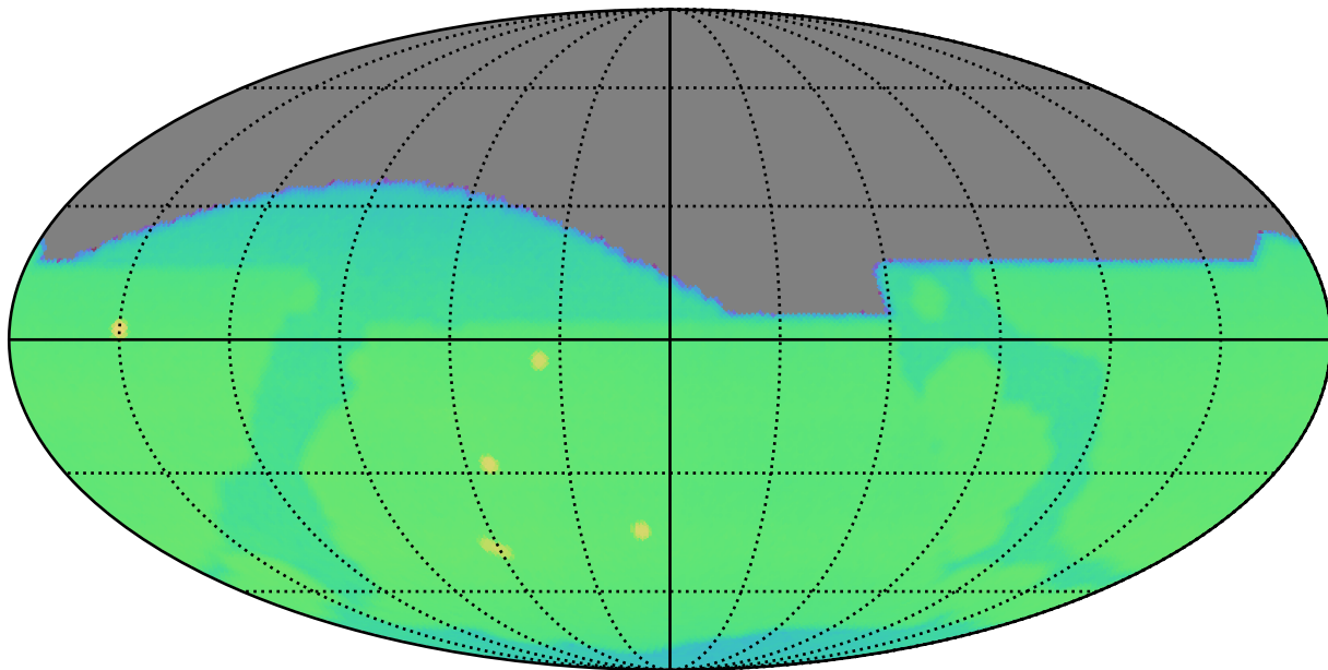
ddf_acor_sf10_lsf30_lsr20_v3.4_10yrs : CoaddM5
