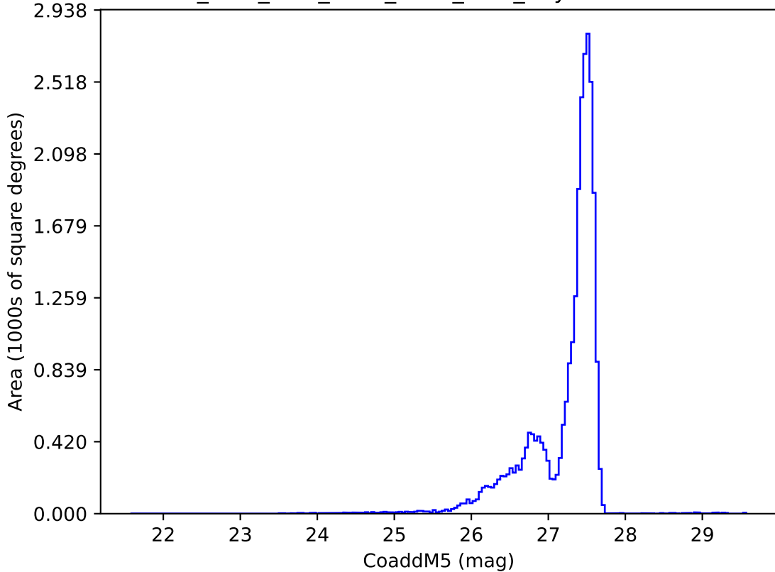
ddf_acor_sf10_lsf30_lsr20_v3.4_10yrs : CoaddM5
