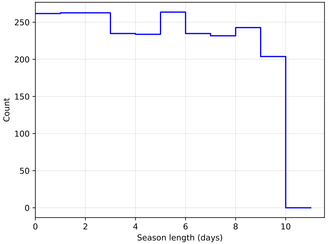
ddf_acor_sf10_lsf30_lsr20_v3.4_10yrs DD:ECDFS all bands: SeasonLength
