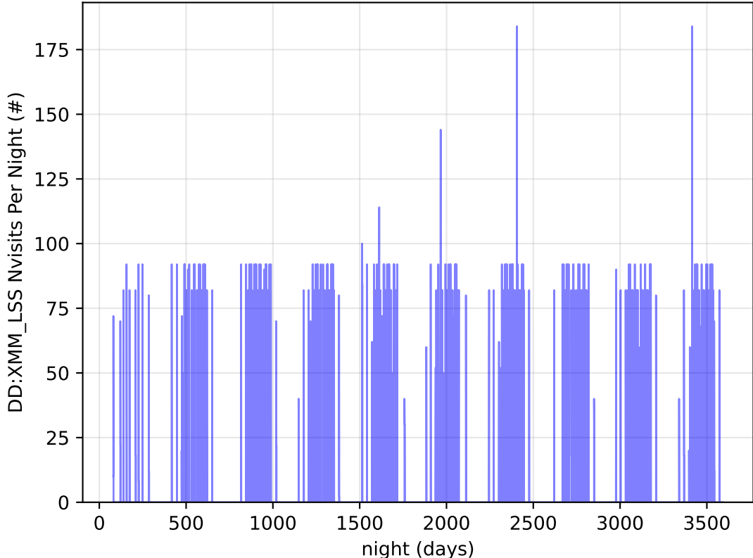
ddf_acor_sf10_lsf30_lsr20_v3.4_10yrs all bands: DD:XMM_LSS Nvisits Per Night
