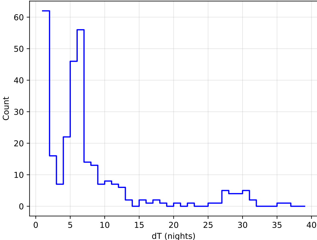
ddf_acor_sf10_lsf30_lsr20_v3.4_10yrs all bands: DD:XMM_LSS Delta Nights Histogram
