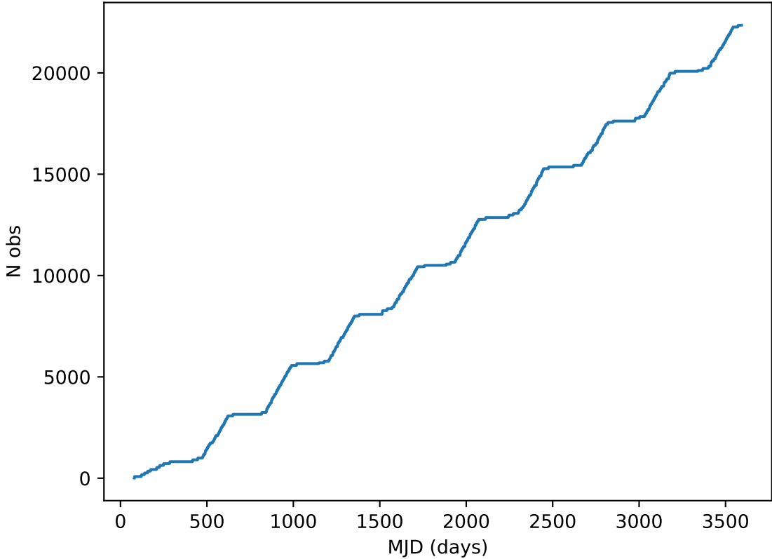
ddf_acor_sf10_lsf30_lsr20_v3.4_10yrs all bands: DD:XMM_LSS Cumulative NVisits
