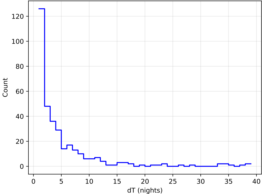
ddf_acor_sf10_lsf30_lsr20_v3.4_10yrs all bands: DD:WFD Delta Nights Histogram
