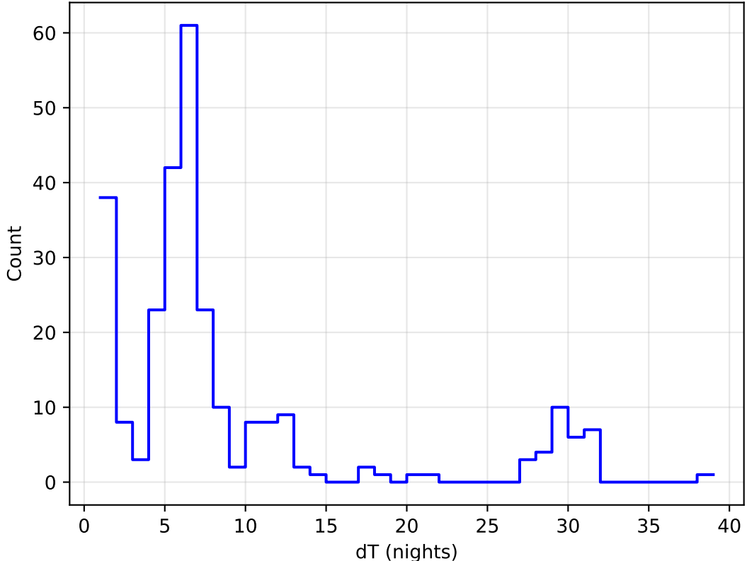
ddf_acor_sf10_lsf30_lsr20_v3.4_10yrs all bands: DD:ELAISS1 Delta Nights Histogram
