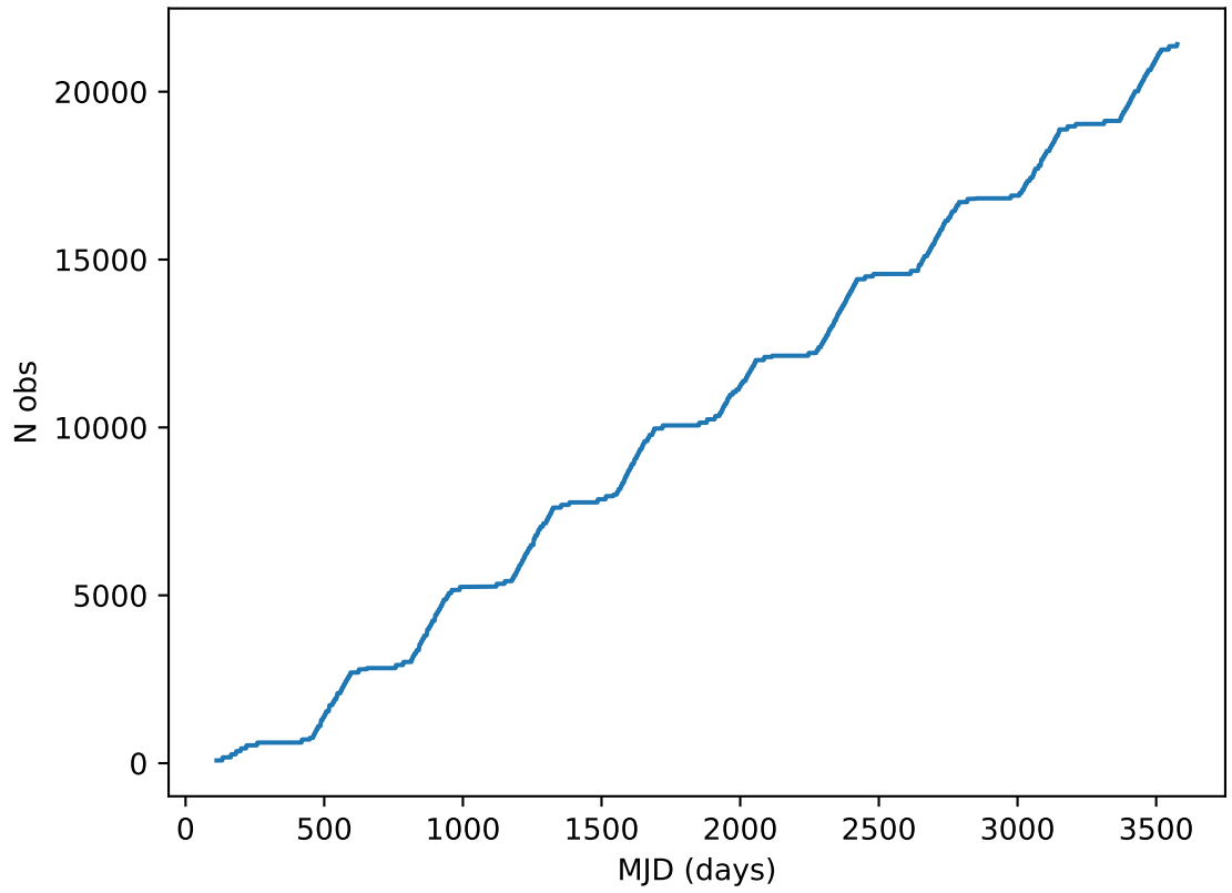
ddf_acor_sf10_lsf30_lsr20_v3.4_10yrs all bands: DD:ELAISS1 Cumulative NVisits
