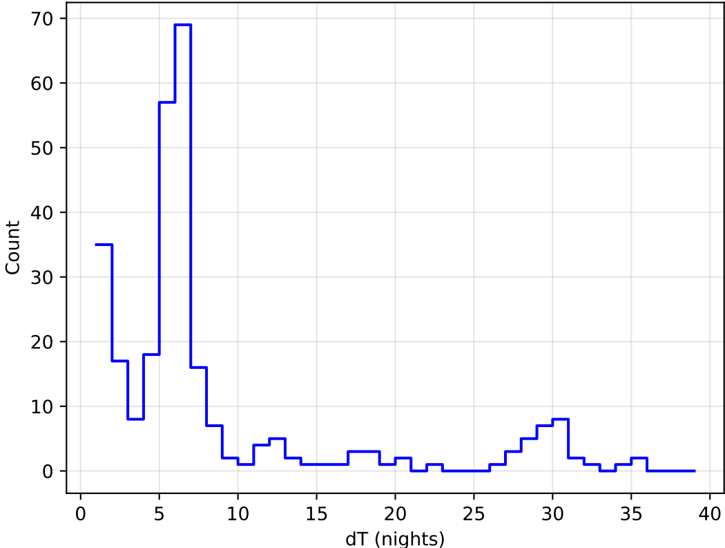
ddf_acor_sf10_lsf30_lsr20_v3.4_10yrs all bands: DD:EDFS Delta Nights Histogram
