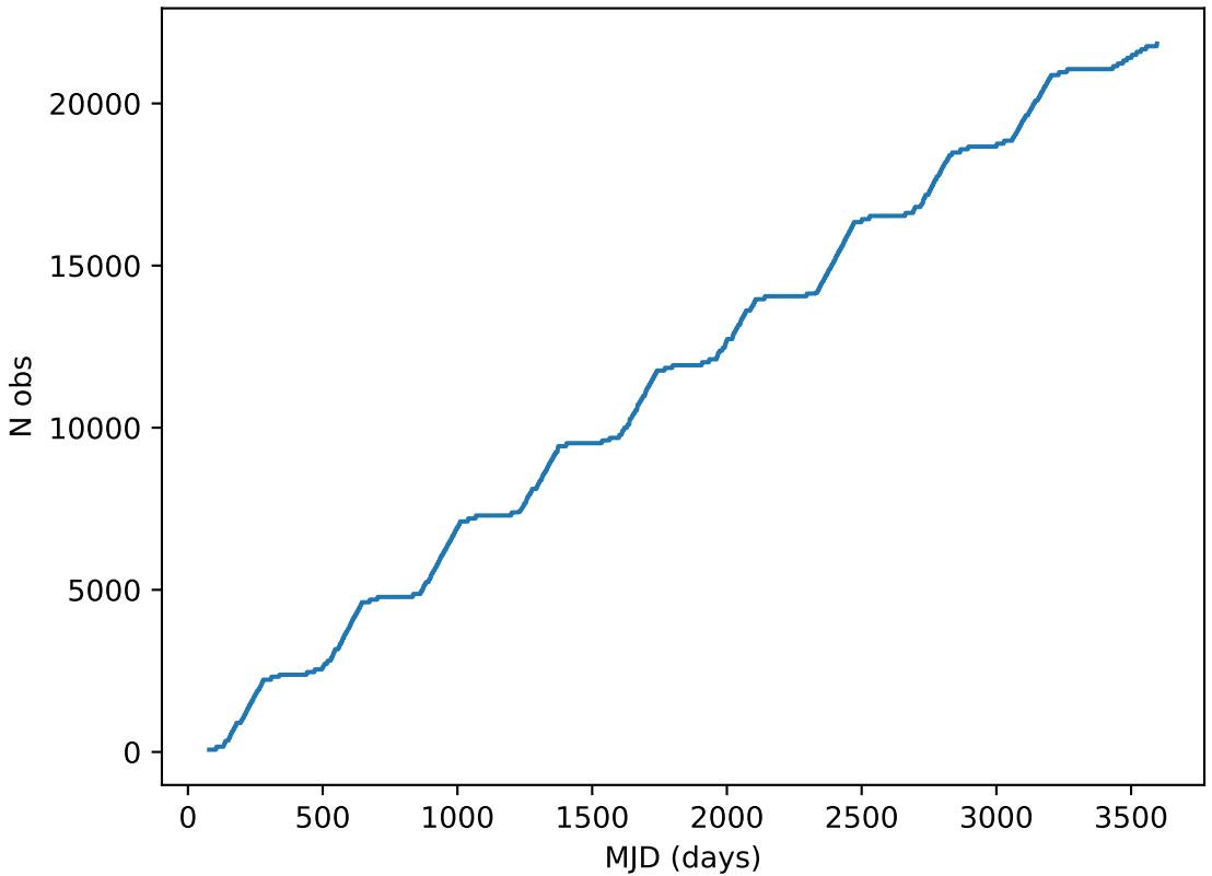
ddf_acor_sf10_lsf30_lsr20_v3.4_10yrs all bands: DD:EDFS Cumulative NVisits
