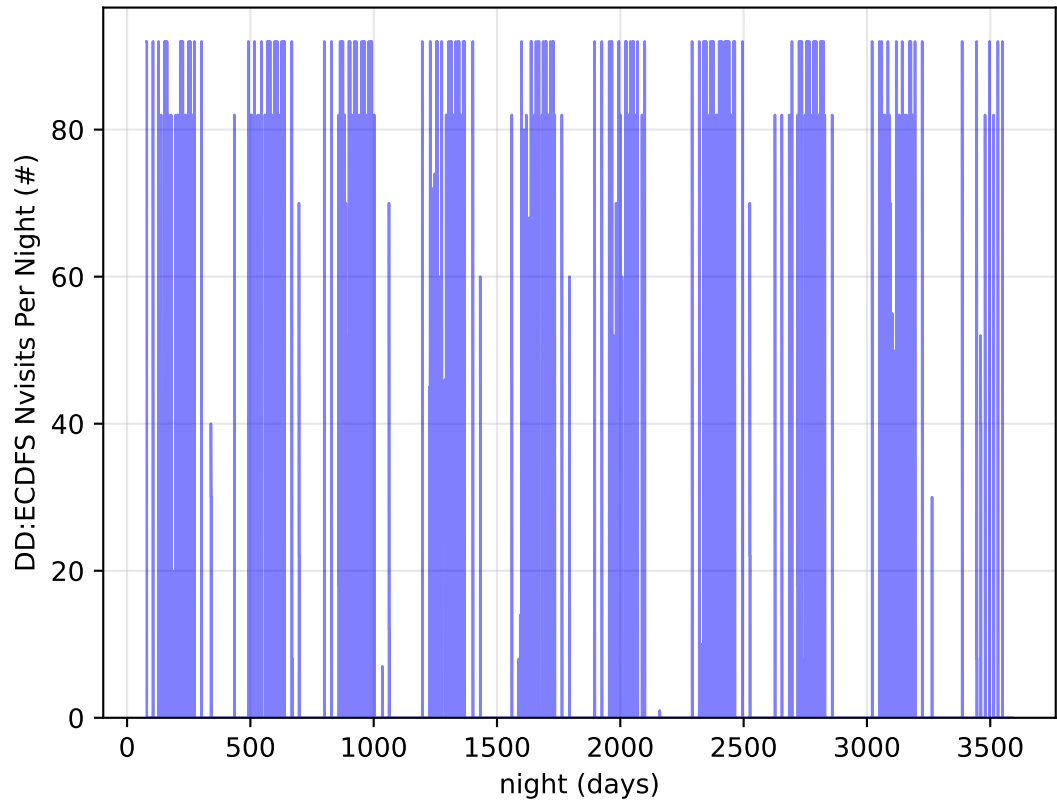
ddf_acor_sf10_lsfs30_lsr20_v3.4_10yrs all bands: DD:ECDFS Nvisits Per Night
