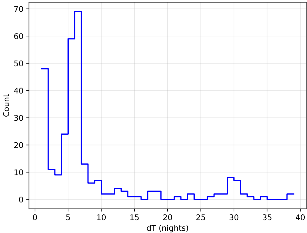
ddf_acor_sf10_lsf30_isr20_v3.4_10yrs all bands: DD:ECDFS Delta Nights Histogram
