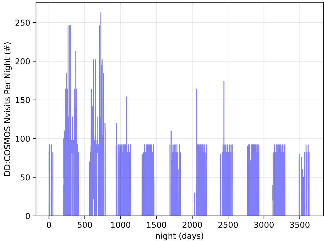
ddf_acor_sf10_lsf30_lsr20_v3.4_10yrs all bands: DD: COSMOS Nvisits Per Night
