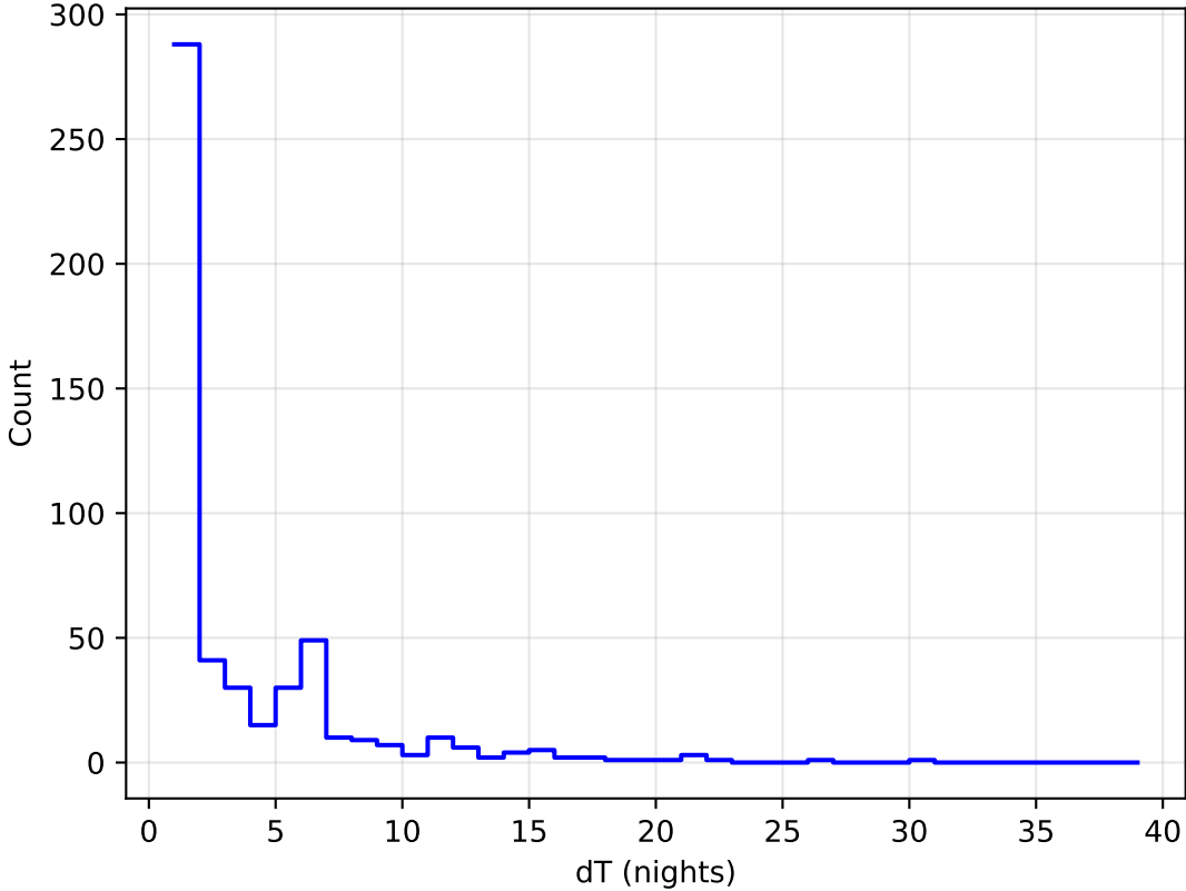
ddf_acor_sf10_Isf30_Isr20_v3.4_10yrs all bands: DD: COSMOS Delta Nights Histogram
