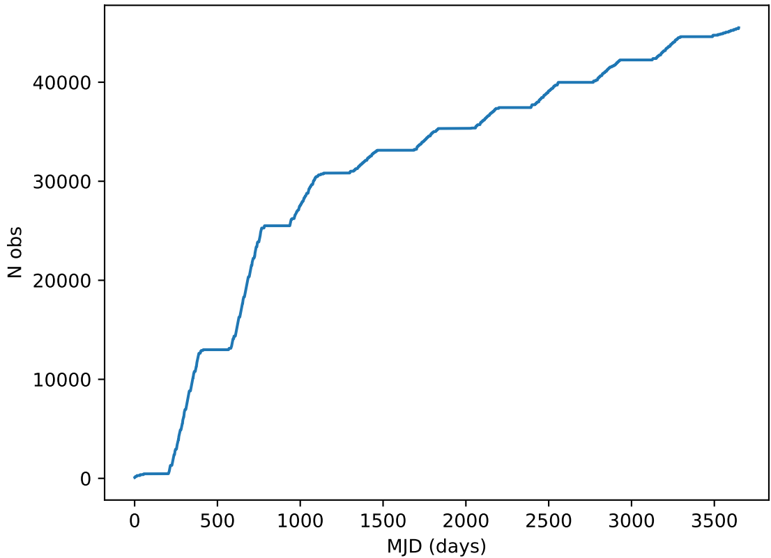
ddf_acor_sf10_lsf30_lsr20_v3.4_10yrs all bands: DD: COSMOS Cumulative NVisits
