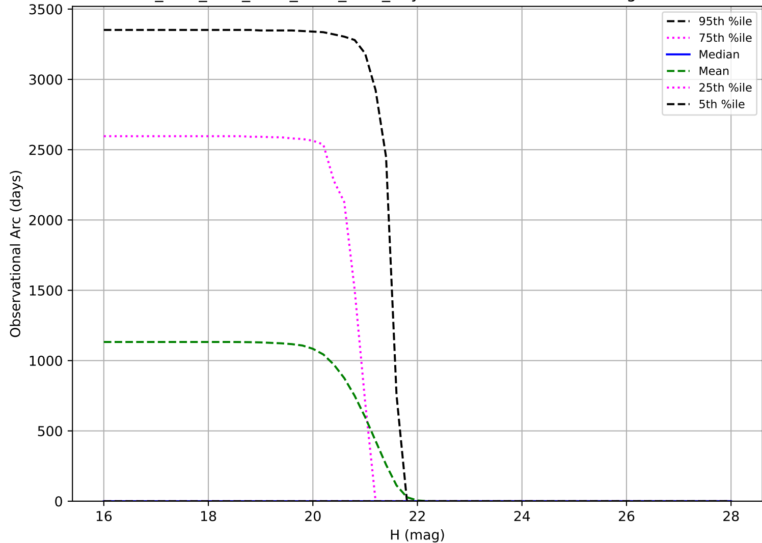
ddf_acor_sf10_lsf30_lsr10_v3.4_10yrs: Observational Arc Length Vatira
