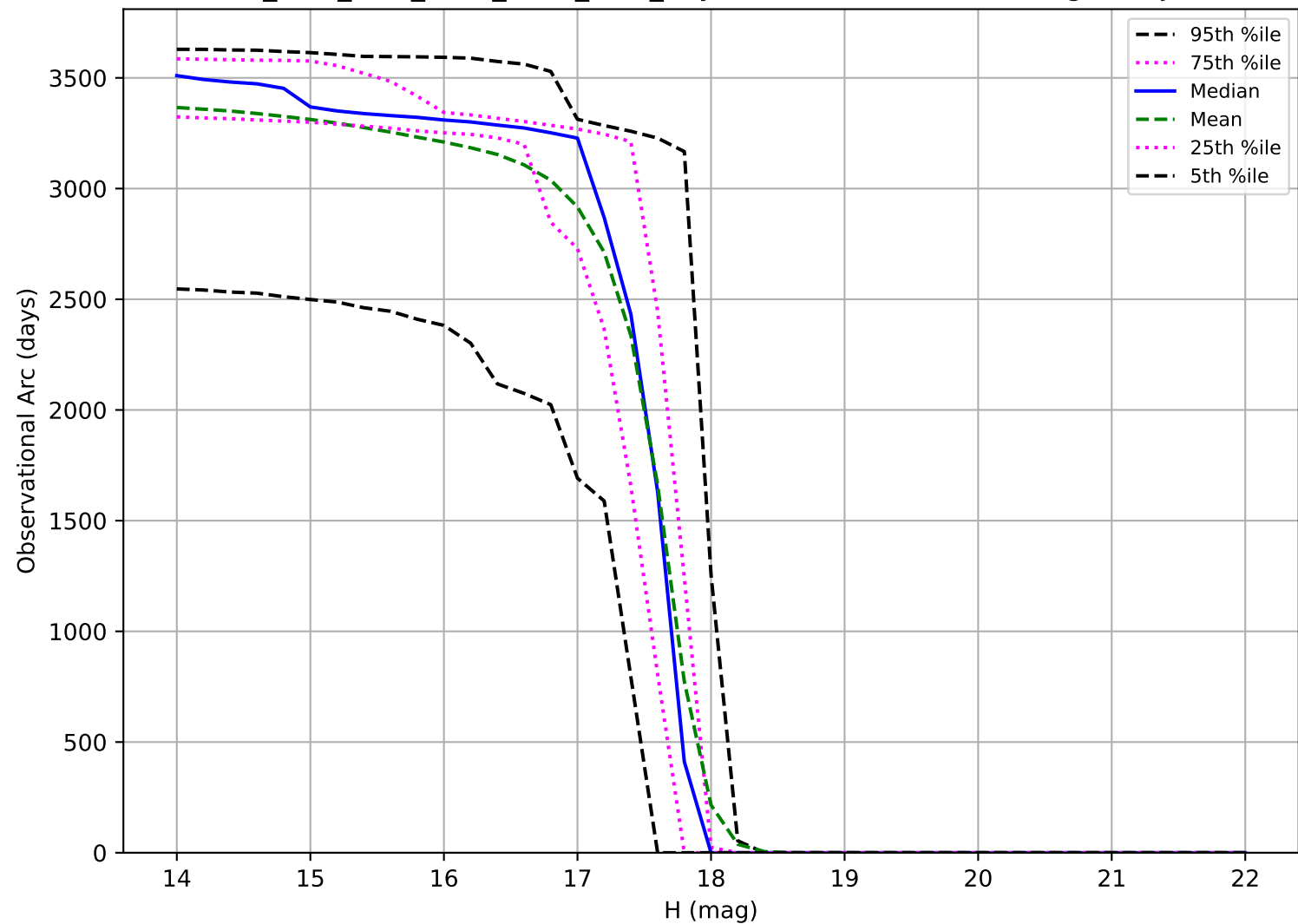
ddf_acor_sf10_lsf30_lsr10_v3.4_10yrs: Observational Arc Length Trojan
