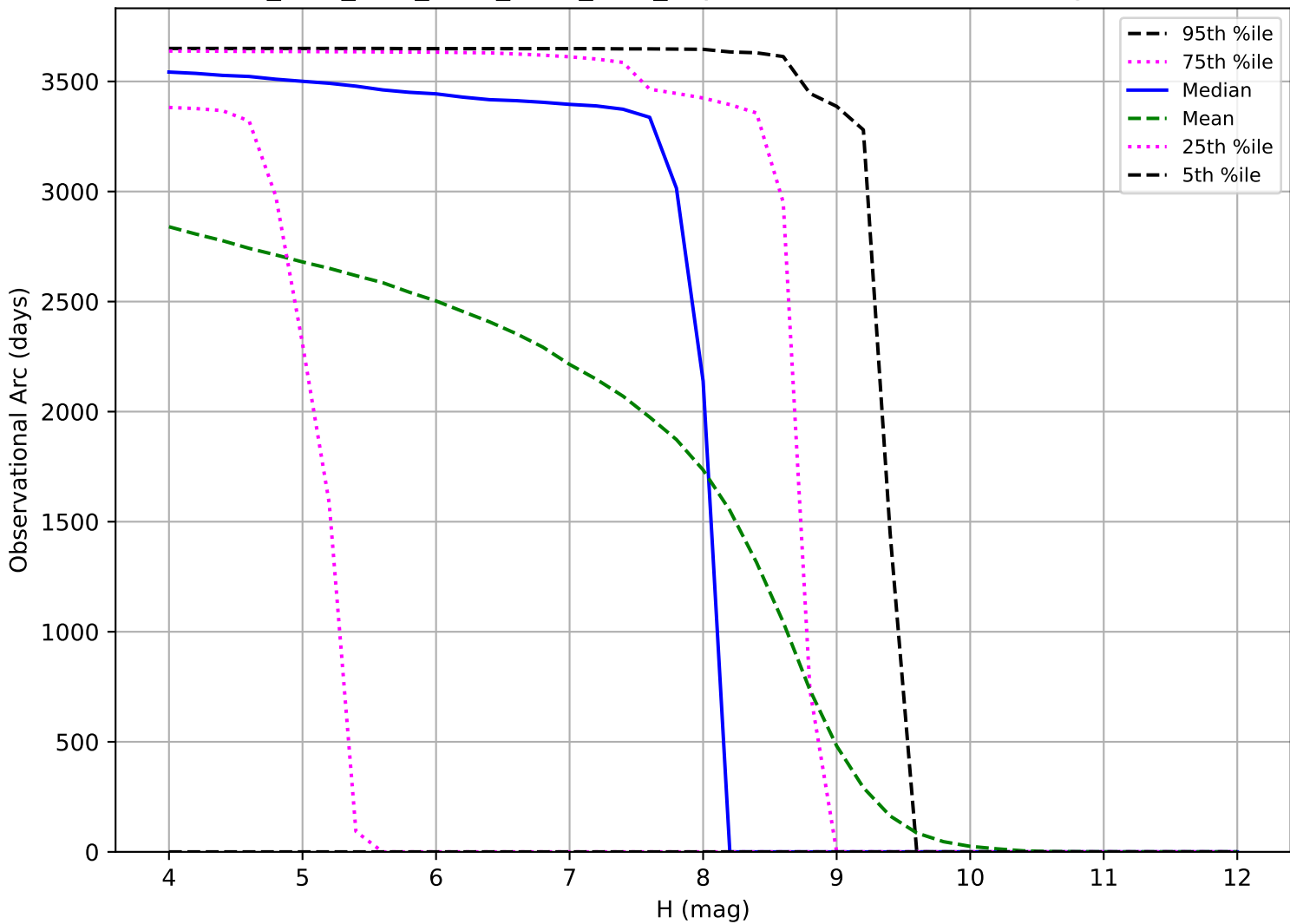
ddf_acor_sf10_lsf30_lsr10_v3.4_10yrs: Observational Arc Length TNO
