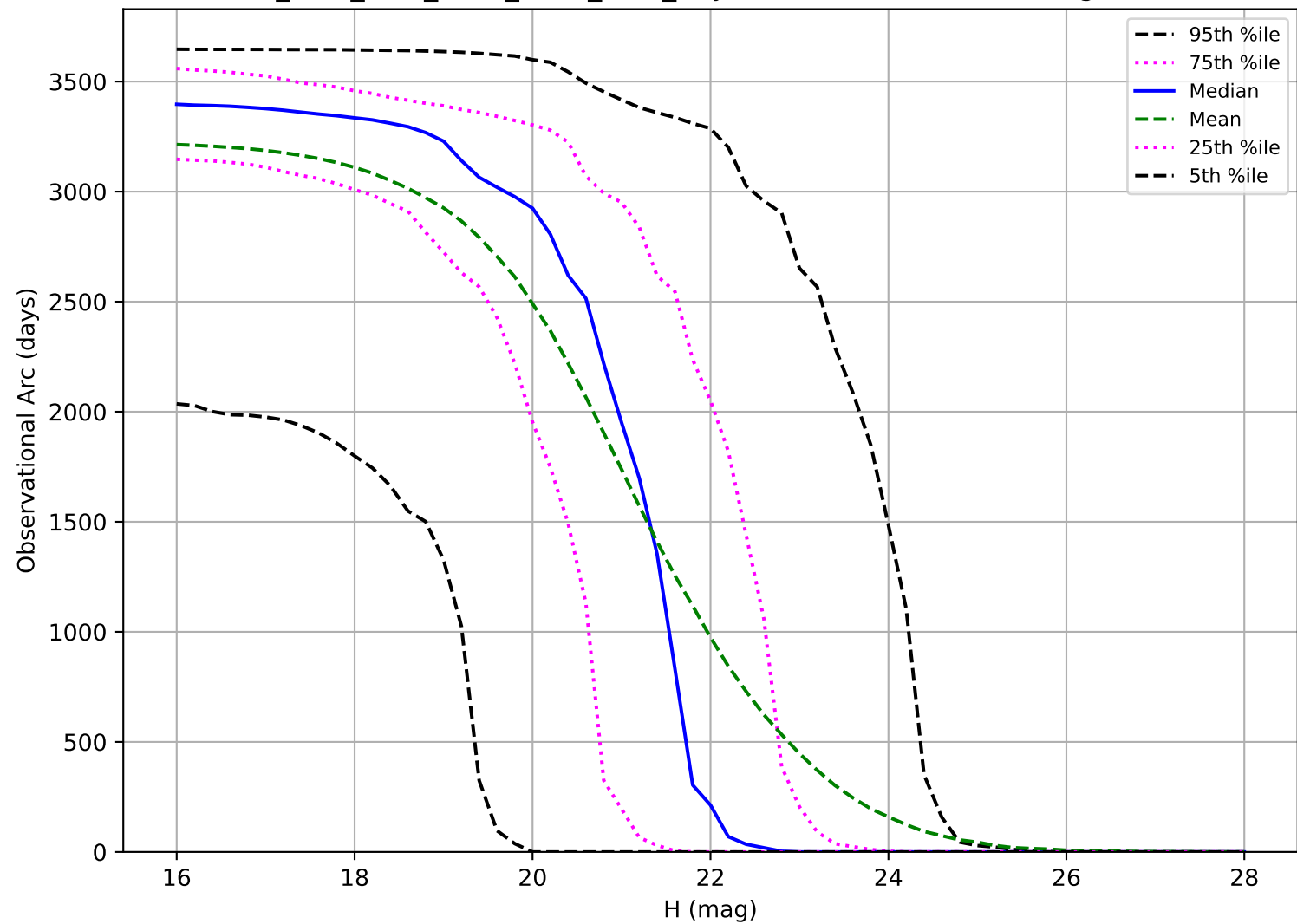
ddf_acor_sf10_lsf30_lsr10_v3.4_10yrs: Observational Arc Length PHA
