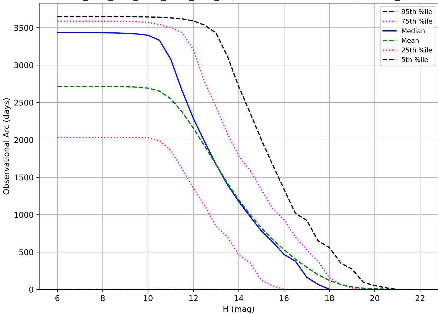
ddf_acor_sf10_lsf30_lsr10_v3.4_10yrs: Observational Arc Length OCC_r5
