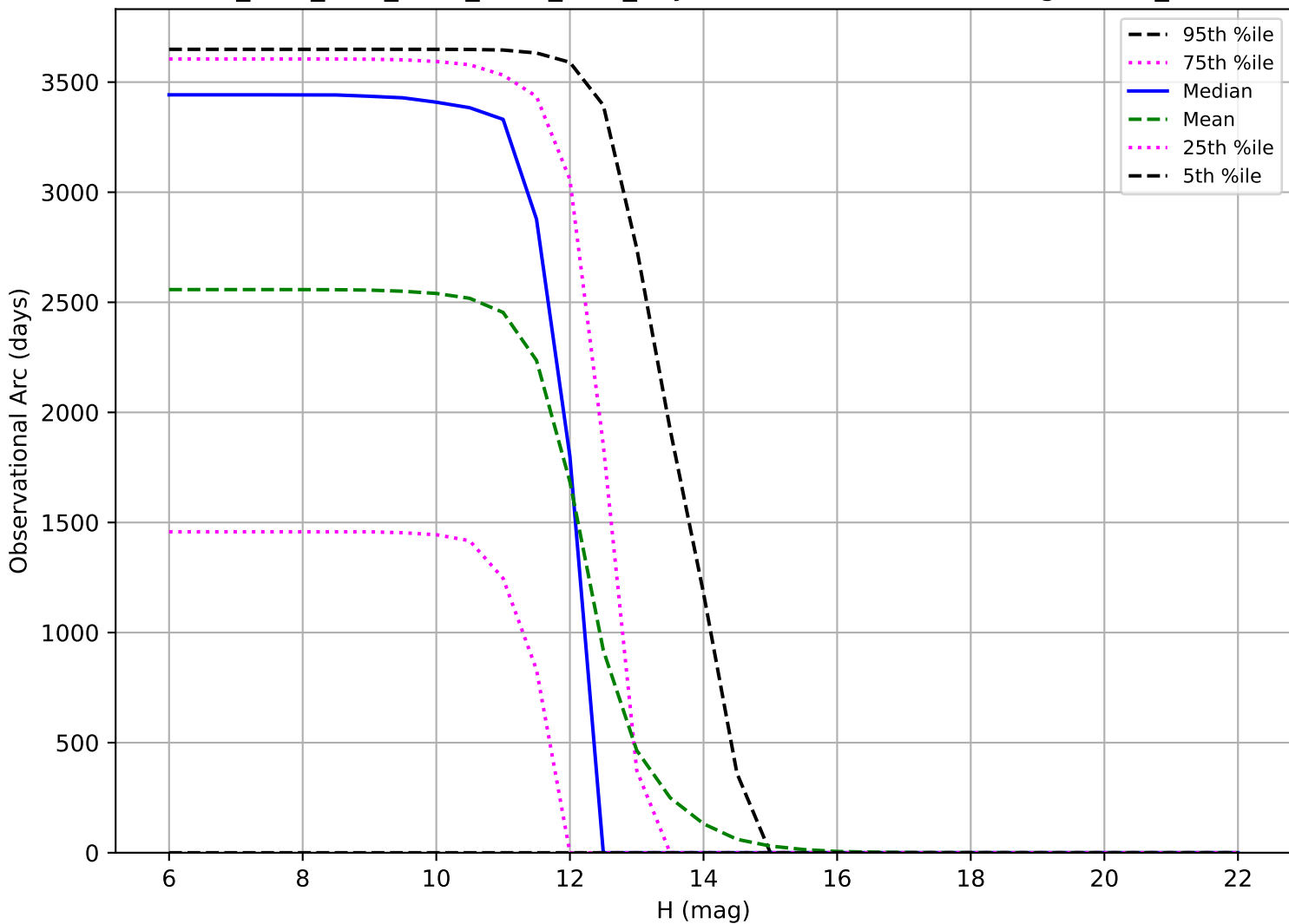
ddf_acor_sf10_lsf30_lsr10_v3.4_10yrs: Observational Arc Length OCC_r20
