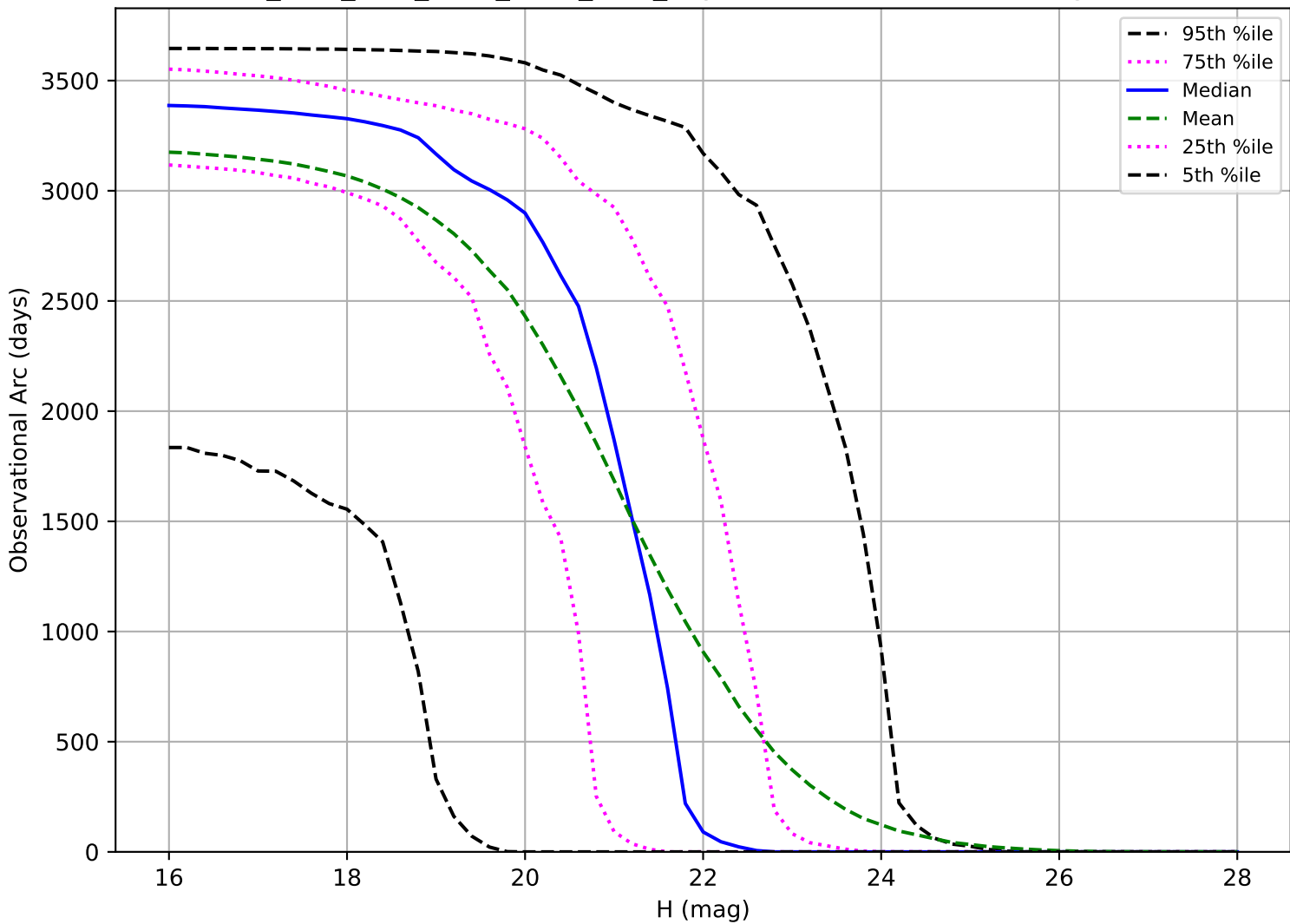
ddf_acor_sf10_lsf30_lsr10_v3.4_10yrs: Observational Arc Length NEO
