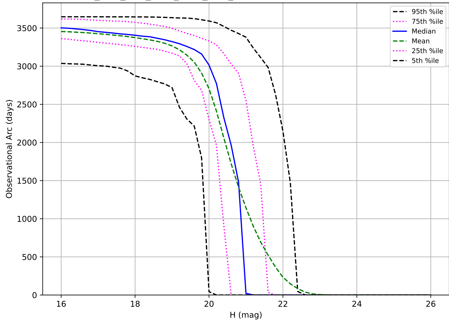
ddf_acor_sf10_lsf30_lsr10_v3.4_10yrs: Observational Arc Length MBA
