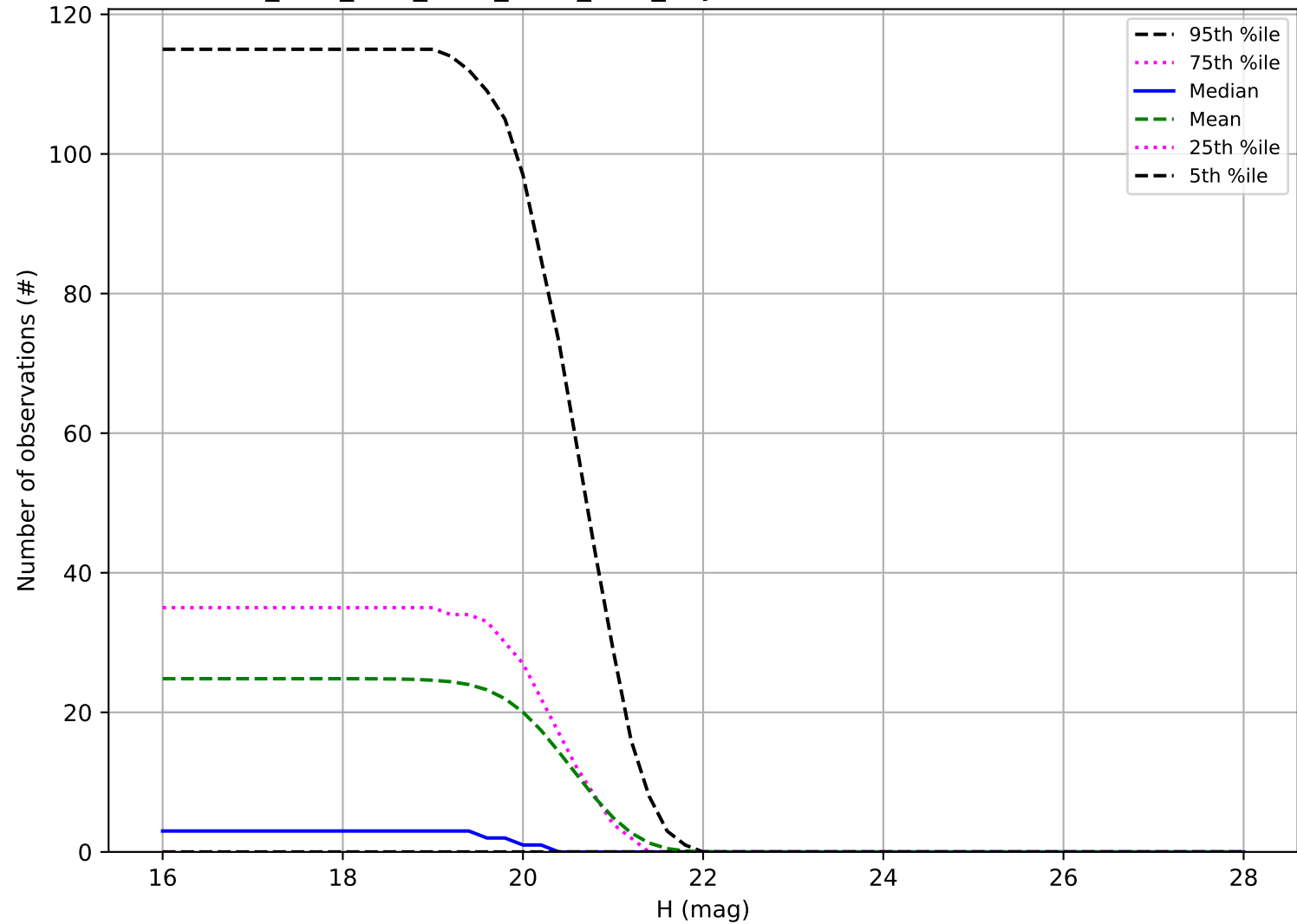
ddf_acor_sf10_lsf30_lsr10_v3.4_10yrs: Number of observations Vatira
