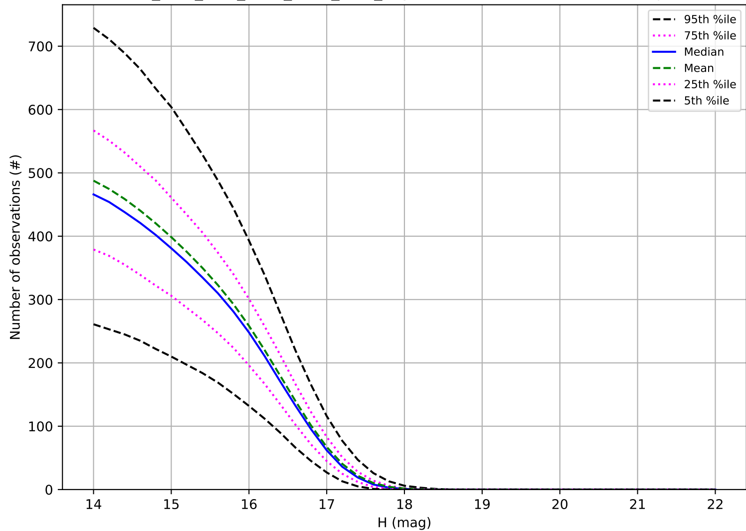
ddf_acor_sf10_lsf30_lsr10_v3.4_10yrs: Number of observations Trojan
