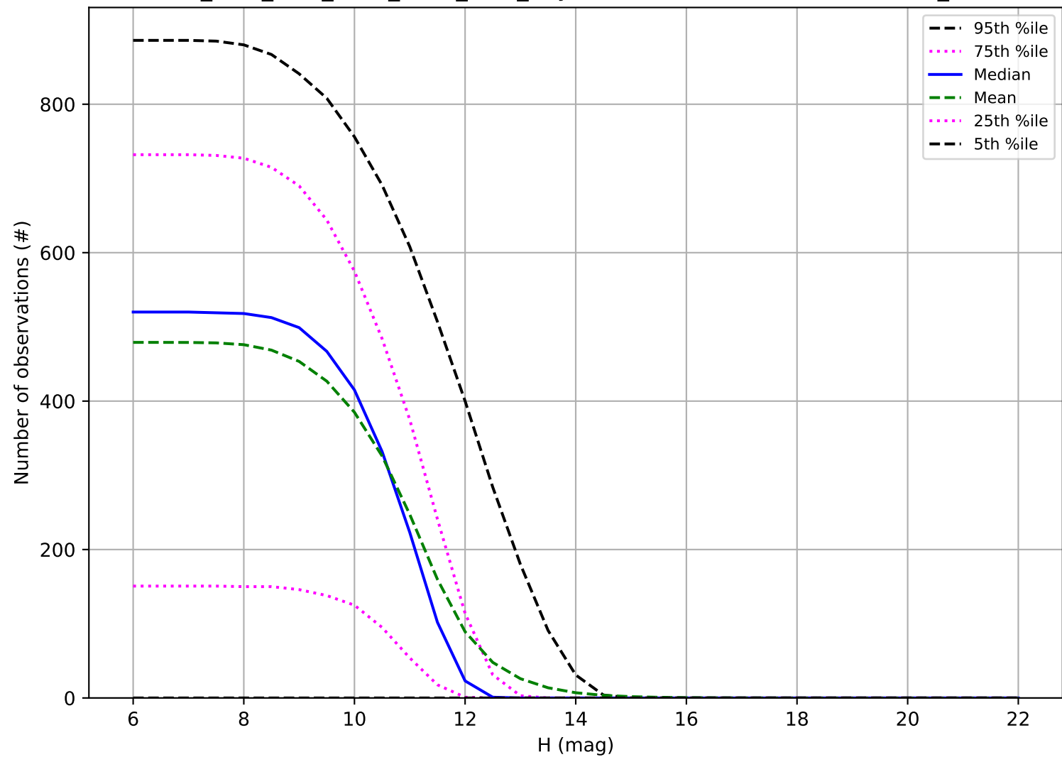
ddf_acor_sf10_lsf30_lsr10_v3.4_10yrs: Number of observations OCC_r20
