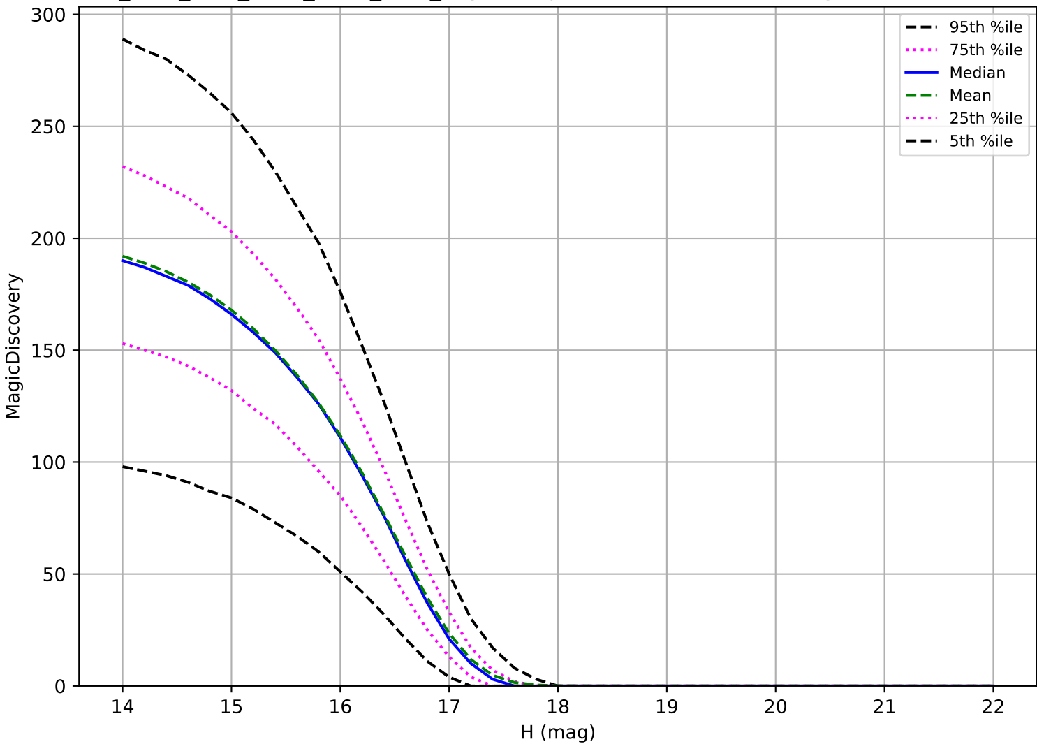
ddf_acor_sf10_lsf30_lsr10_v3.4_10yrs: Trojan 6 detections in 60 nights detection loss
