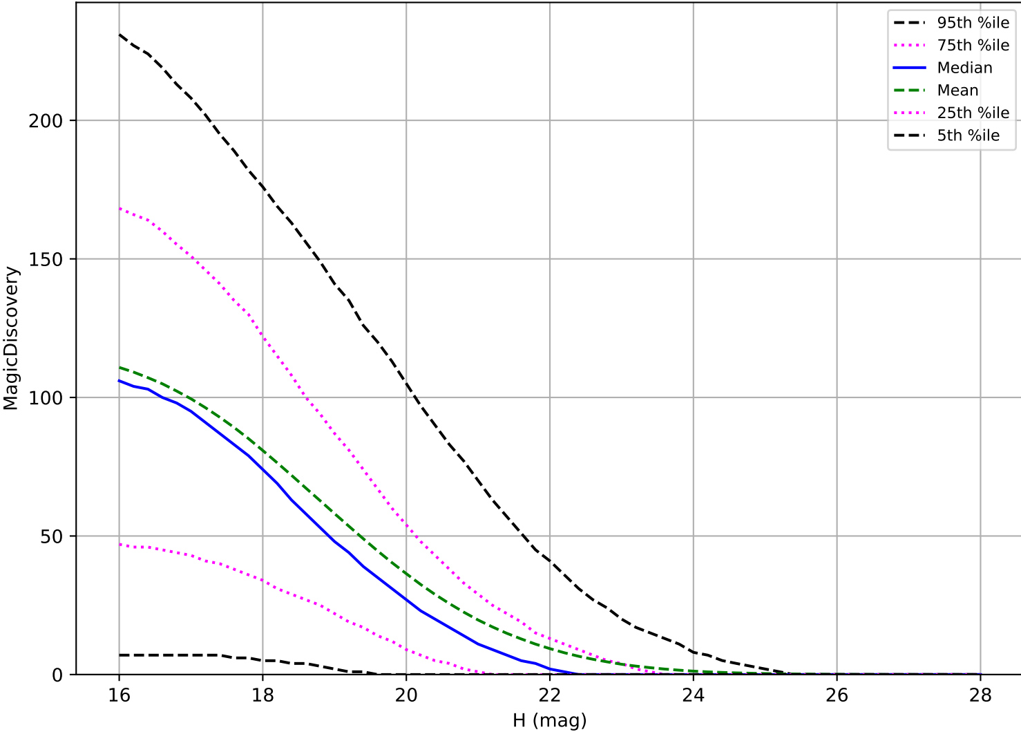
ddf_acor_sf10_lsf30_lsr10_v3.4_10yrs: PHA 6 detections in 60 nights detection loss
