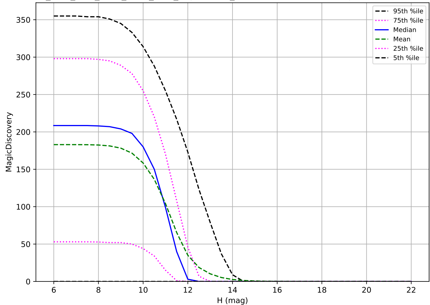
ddf_acor_sf10_lsf30_lsr10_v3.4_10yrs: OCC_r20 6 detections in 60 nights detection loss
