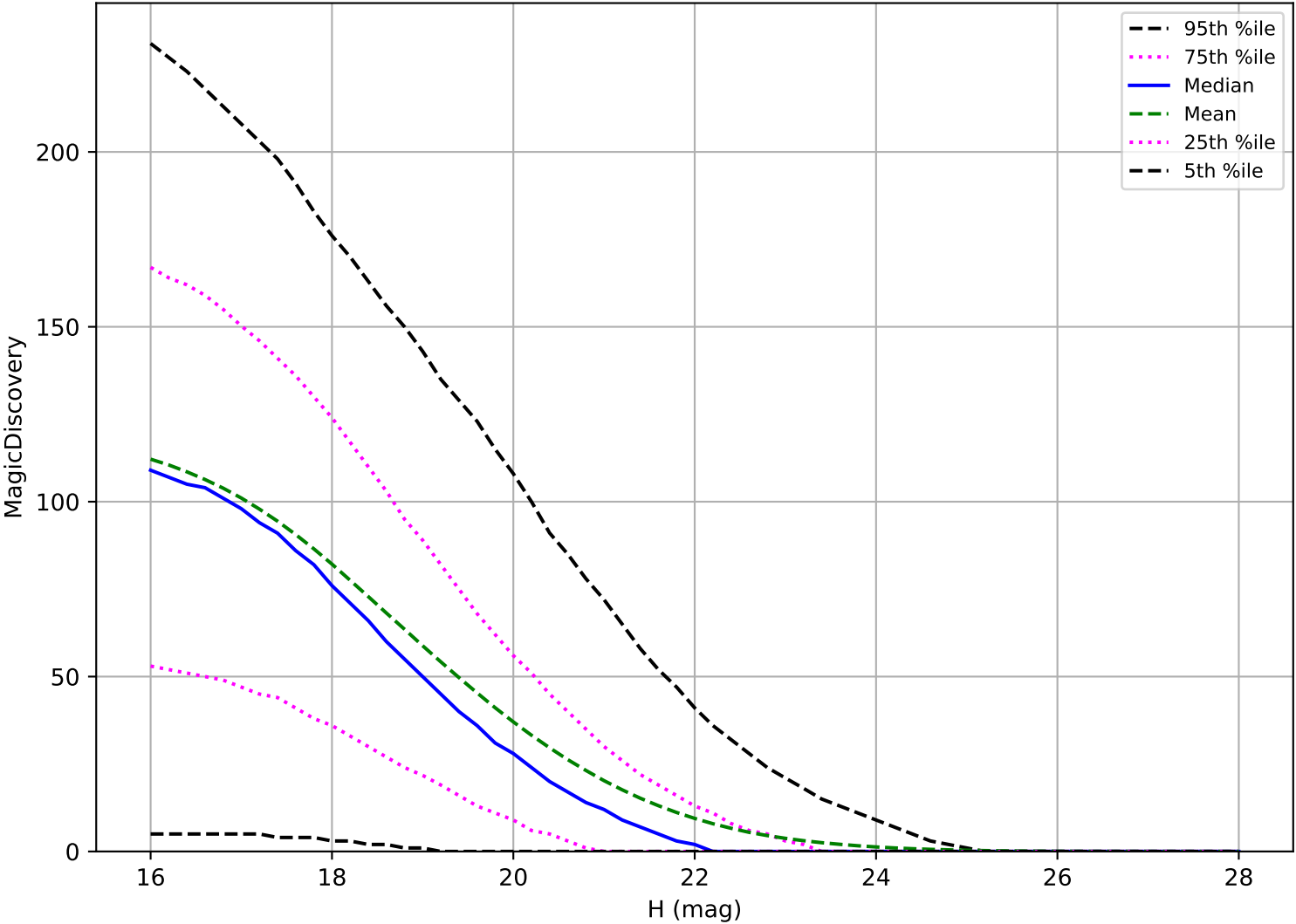
ddf_acor_sf10_lsf30_lsr10_v3.4_10yrs: NEO 6 detections in 60 nights detection loss
