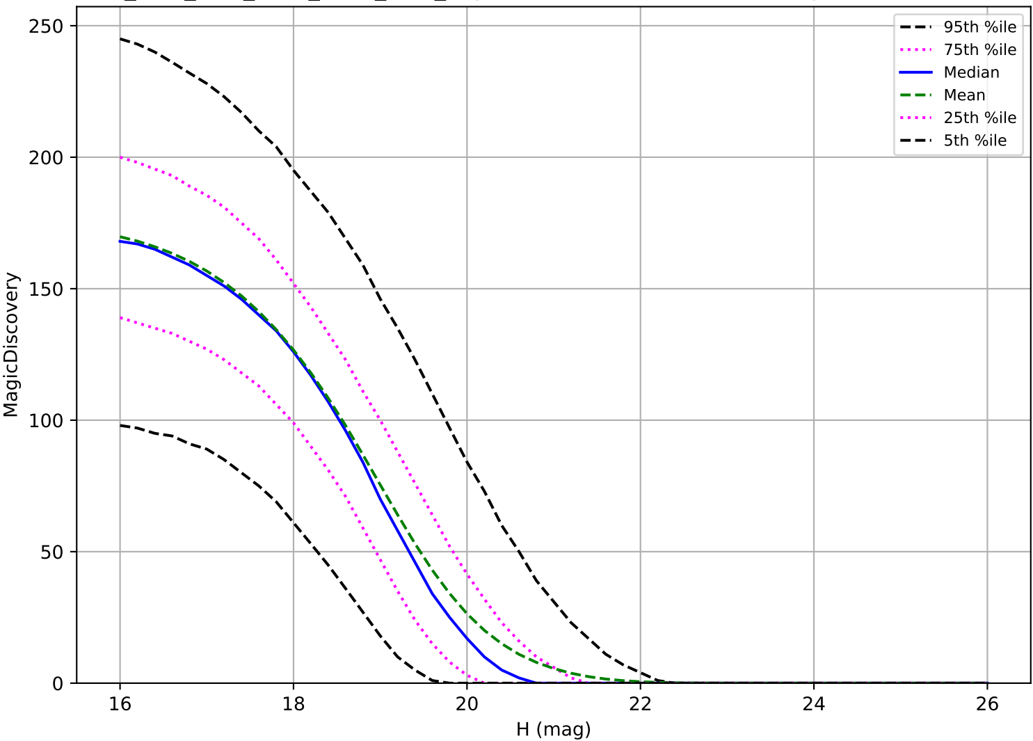
ddf_acor_sf10_lsf30_lsr10_v3.4_10yrs: MBA 6 detections in 60 nights detection loss
