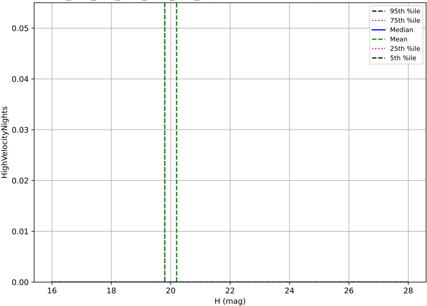
ddf_acor_sf10_lsf30_lsr10_v3.4_10yrs: Vatira High velocity pair detection loss
