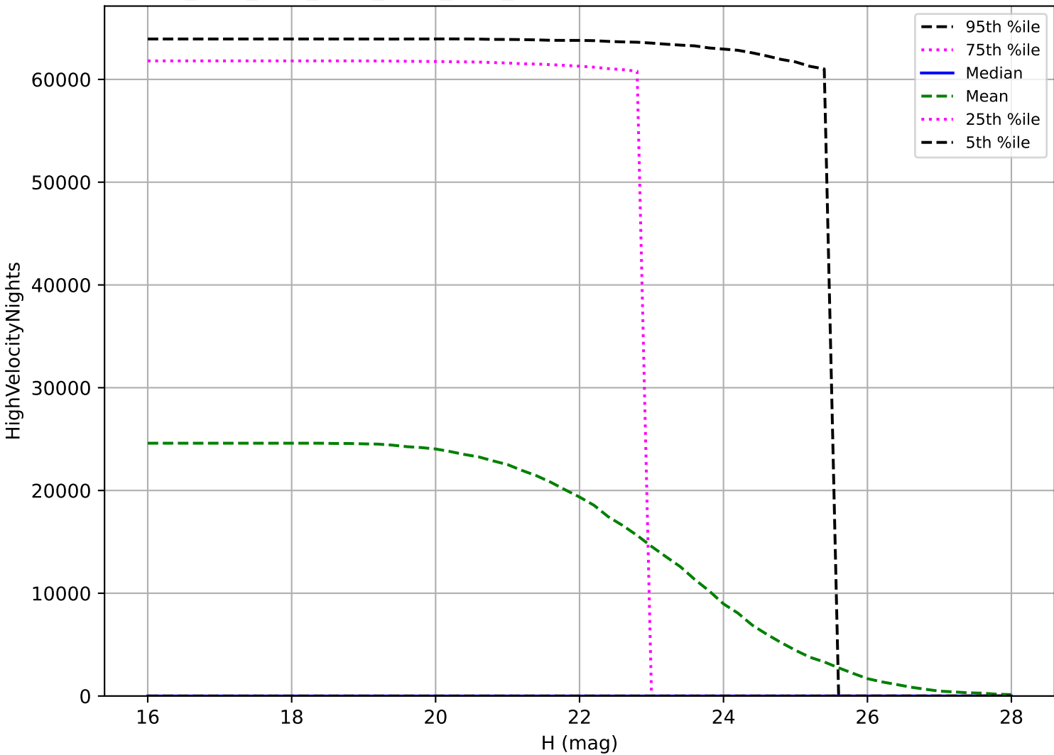
ddf_acor_sf10_lsf30_lsr10_v3.4_10yrs: PHA High velocity pair detection loss
