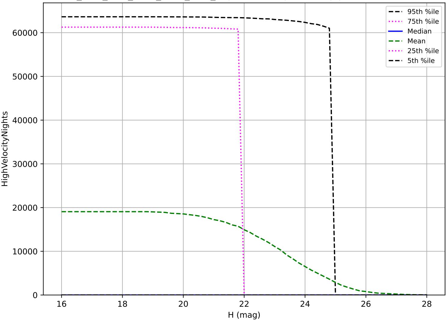
ddf_acor_sf10_lsf30_lsr10_v3.4_10yrs: NEO High velocity pair detection loss
