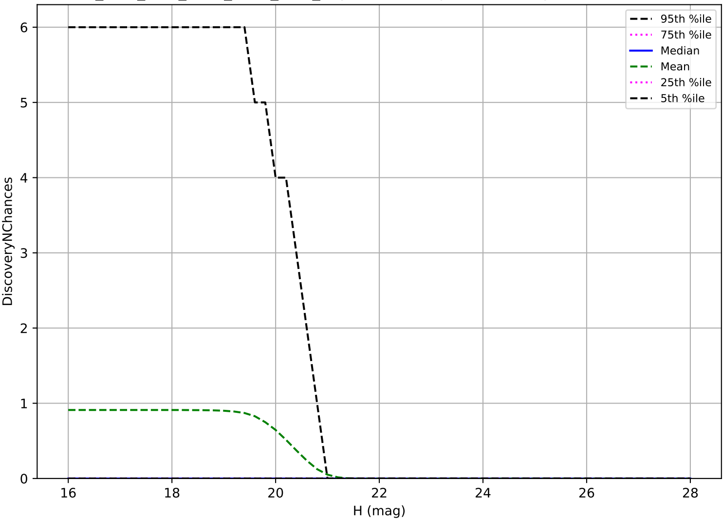
ddf_acor_sf10_lsf30_lsr10_v3.4_10yrs: Vatira 3 pairs in 15 nights detection loss
