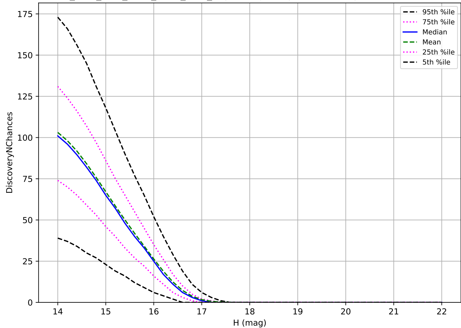
ddf_acor_sf10_lsf30_lsr10_v3.4_10yrs: Trojan 3 pairs in 15 nights detection loss
