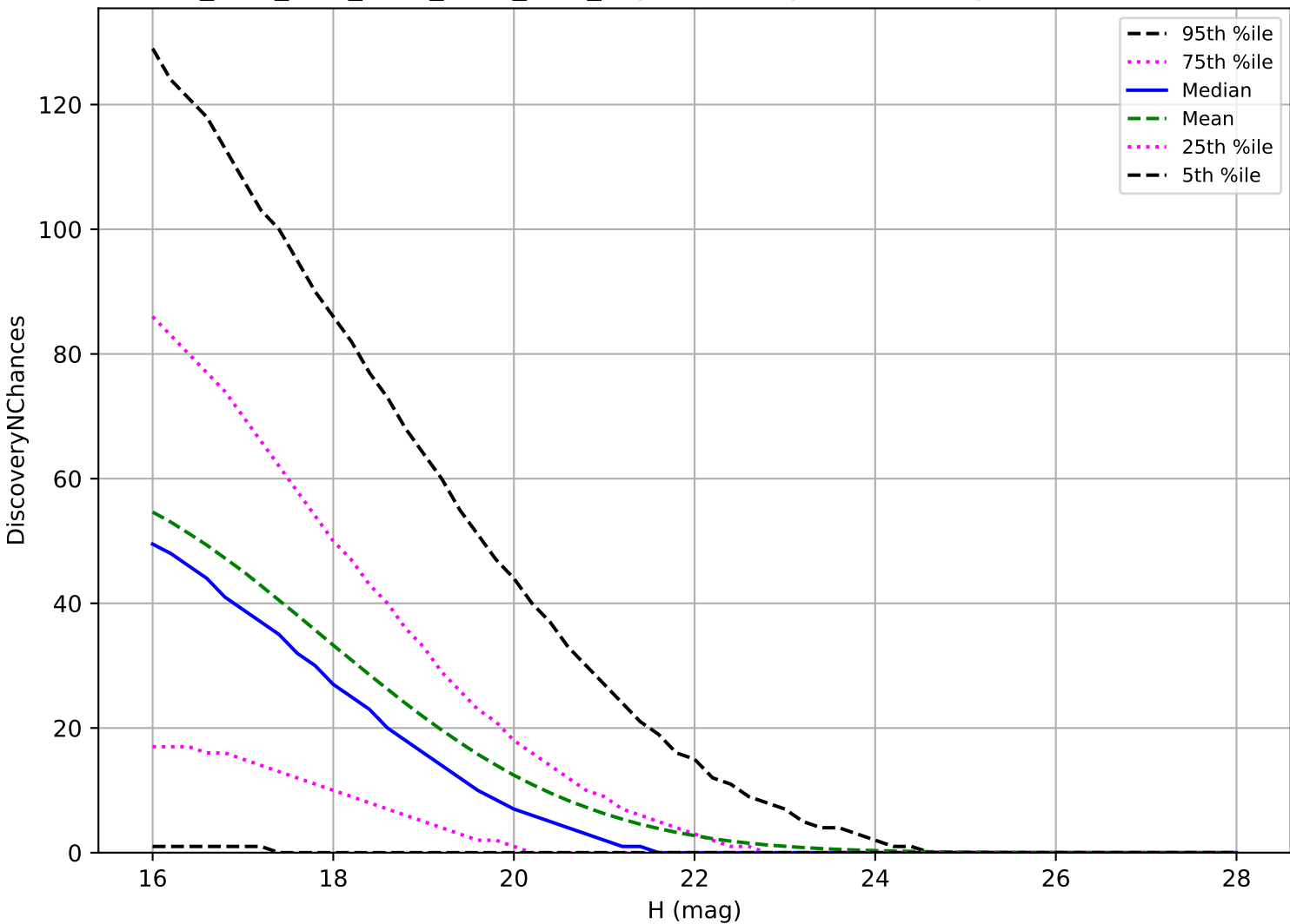
ddf_acor_sf10_lsf30_lsr10_v3.4_10yrs: PHA 3 pairs in 15 nights detection loss
