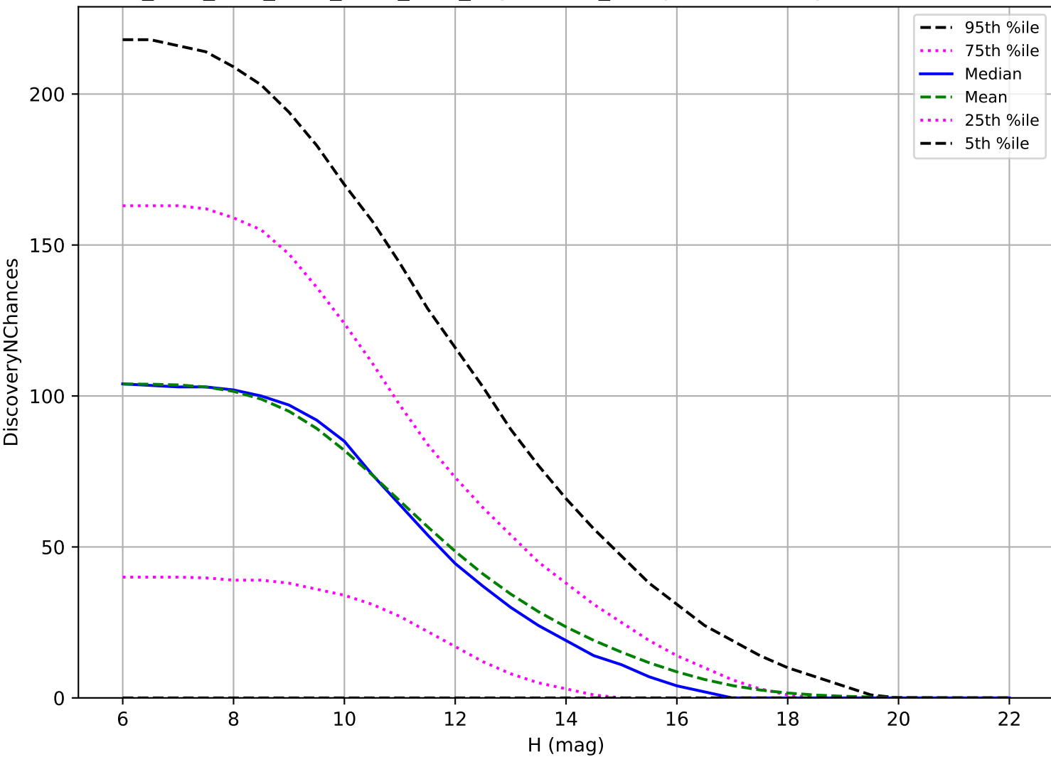
ddf_acor_sf10_lsf30_lsr10_v3.4_10yrs: OCC_r5 3 pairs in 15 nights detection loss
