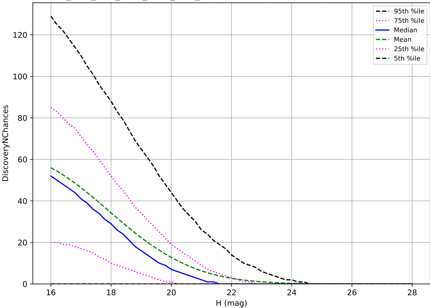
ddf_acor_sf10_lsf30_lsr10_v3.4_10yrs: NEO 3 pairs in 15 nights detection loss
