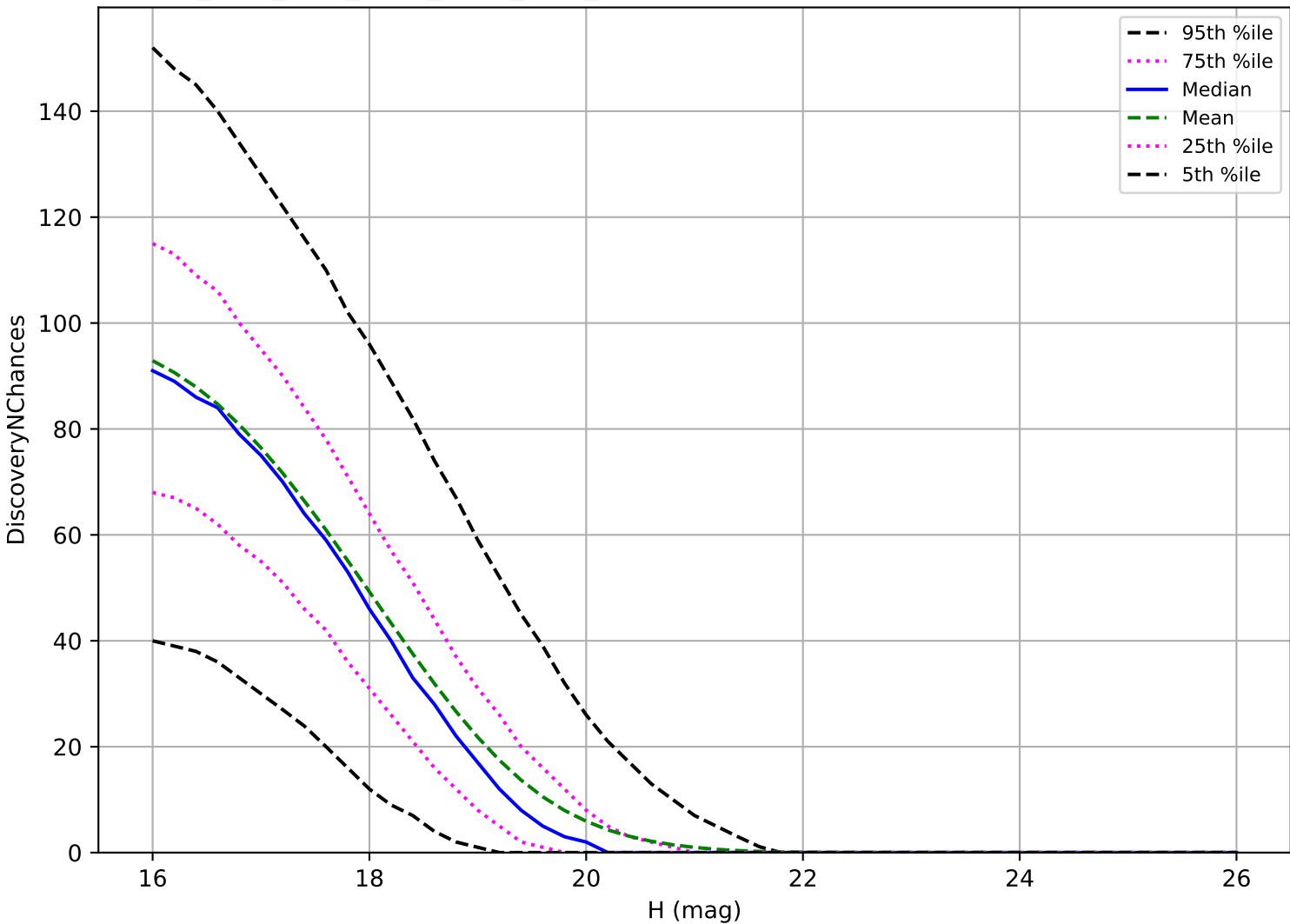
ddf_acor_sf10_lsf30_lsr10_v3.4_10yrs: MBA 3 pairs in 15 nights detection loss
