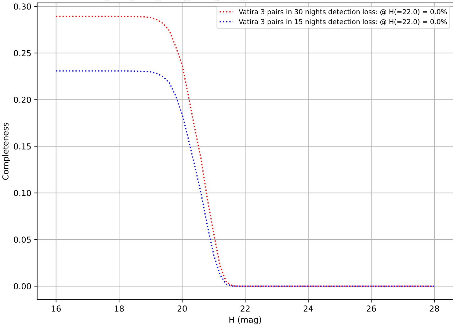
ddf_acor_sf10_lsf30_lsr10_v3.4_10yrs: DifferentialCompleteness
