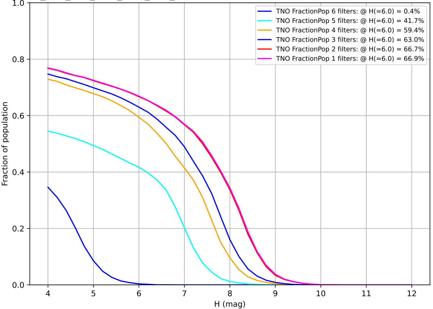
ddf_acor_sf10_lsf30_lsr10_v3.4_10yrs: Fraction of population with colors in X filters TNO
