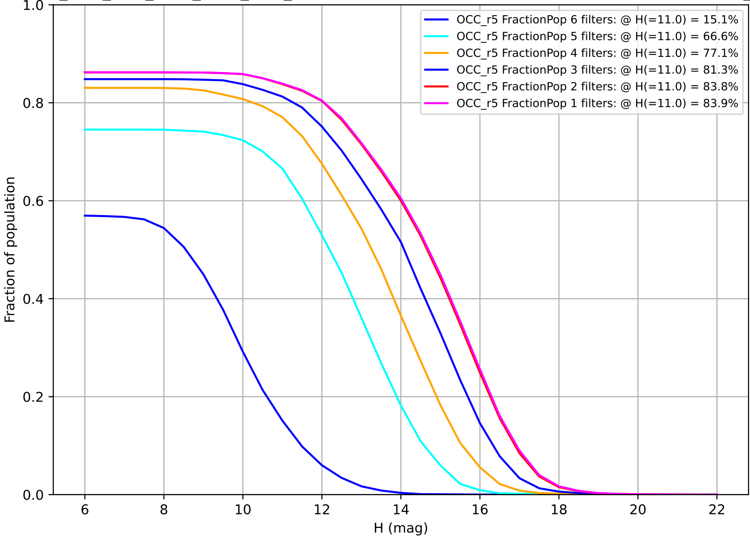
ddf_acor_sf10_lsf30_lsr10_v3.4_10yrs: Fraction of population with colors in X filters OCC_r5
