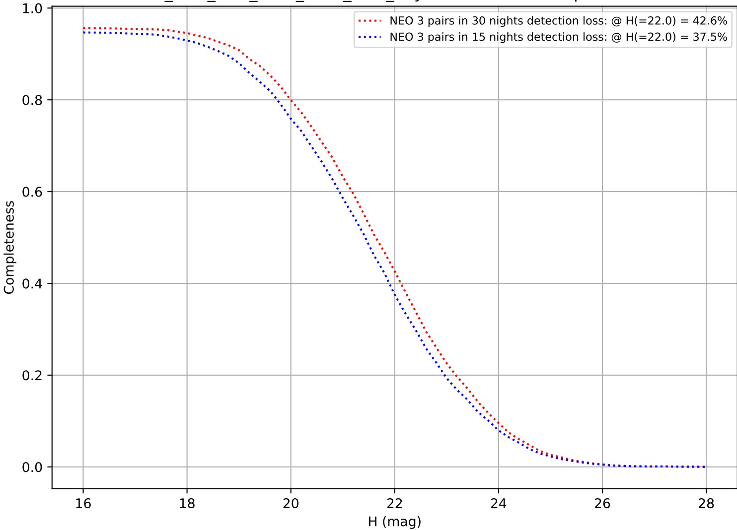
ddf_acor_sf10_lsf30_lsr10_v3.4_10yrs: DifferentialCompleteness
