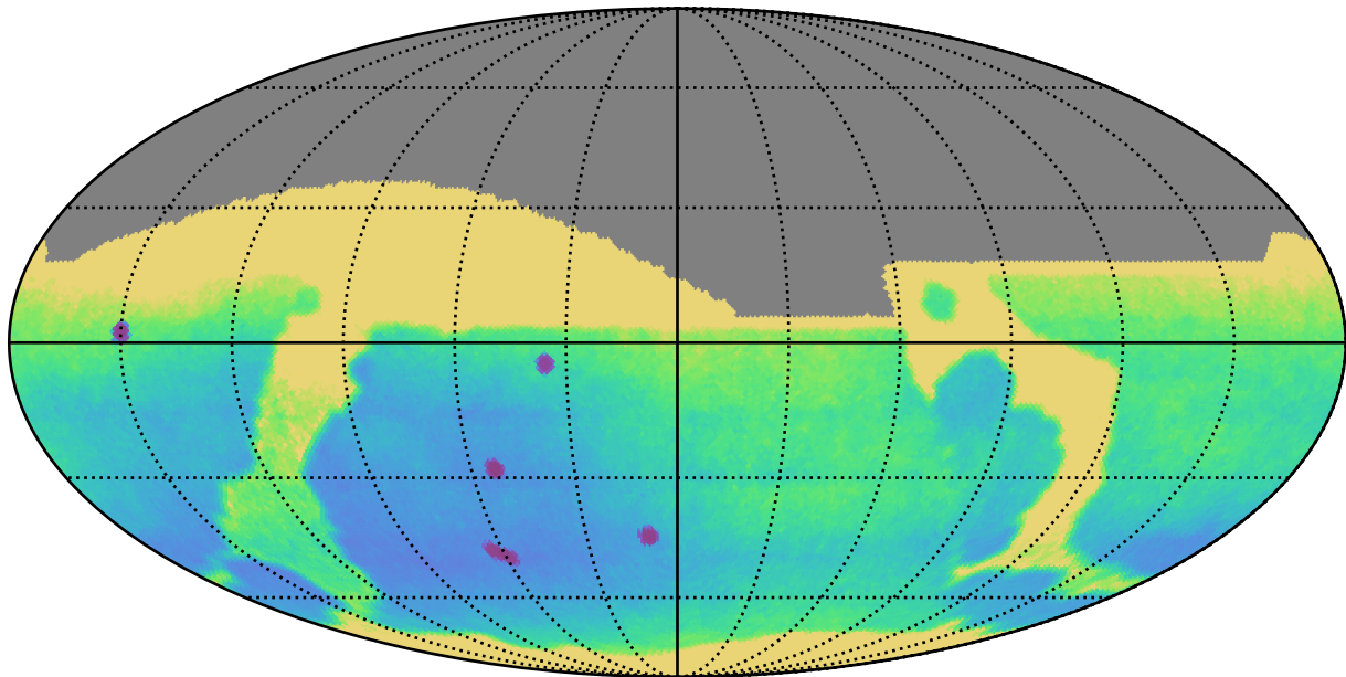
ddf_acor_sf10_lsf30_lsr10_v3.4_10yrs : Parallax Uncert @ 24.0
