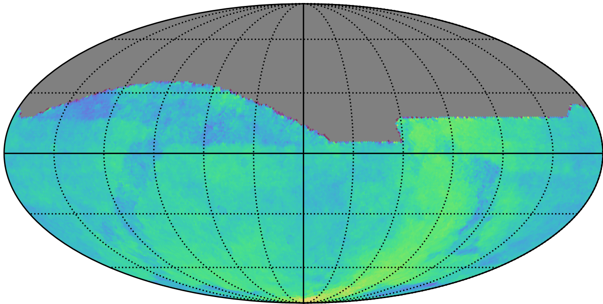
ddf_acor_sf10_lsf30_lsr10_v3.4_10yrs : Parallax Coverage @ 24.0
