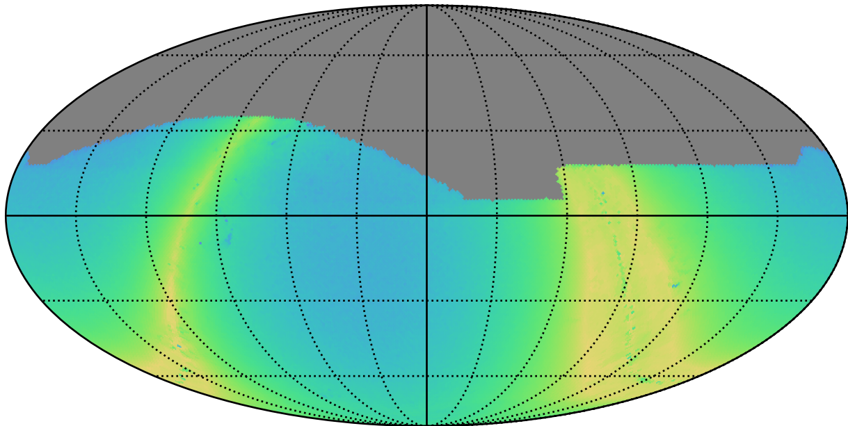
ddf_acor_sf10_lsf30_lsr10_v3.4_10yrs i: N stars to Precision 0.20
