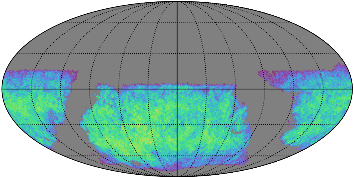
ddf_acor_sf10_lsf30_lsr10_v3.4_10yrs i band non-DD year 1: ExgalM5WithCuts
